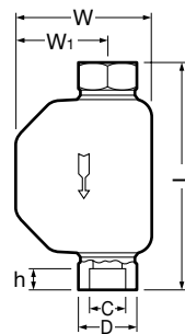
承插焊
