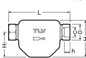
承插焊
